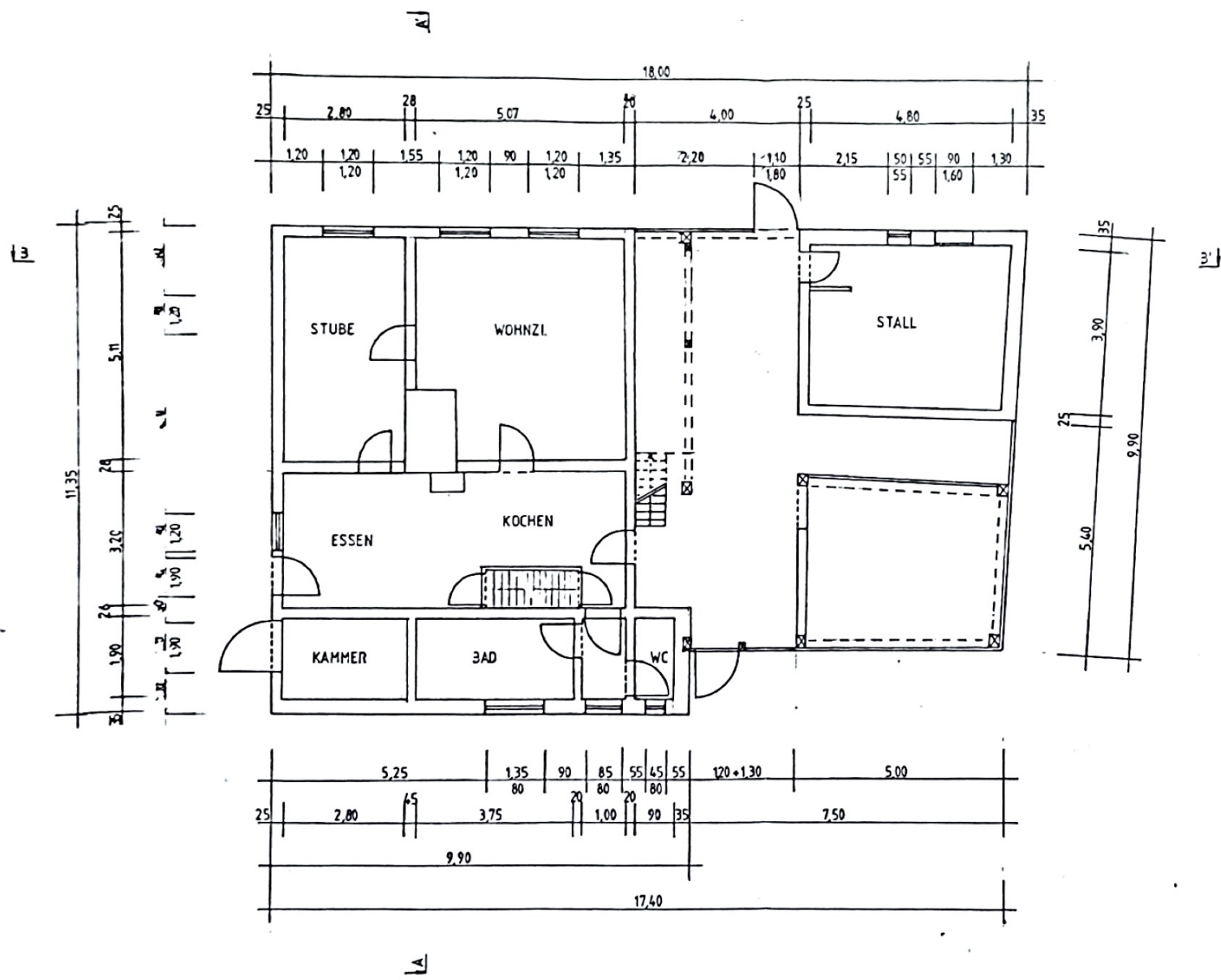
ERDGESCHOSS M. = 1:100
